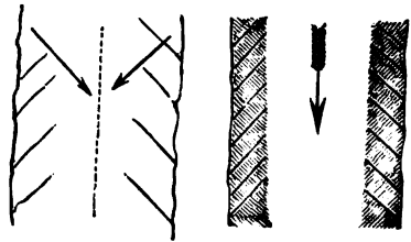
FIG. 6. FIG. 7. FIGS. 6, 7.—Illustrate the formation of marginal fissures and veins.
